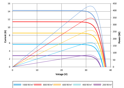
Current-Voltage & Power-Voltage Curve (430S)
